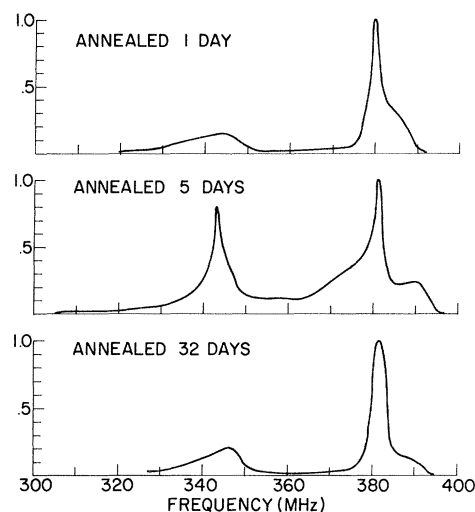
FIG. 2. Uncorrected \text{Mn}^{55} line shapes at 77°K. The unannealed signal was too weak to observe.
