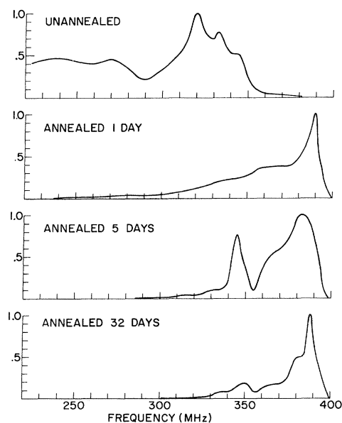
FIG. 1. Uncorrected \text{Mn}^{55} line shapes at 4.2°K.
